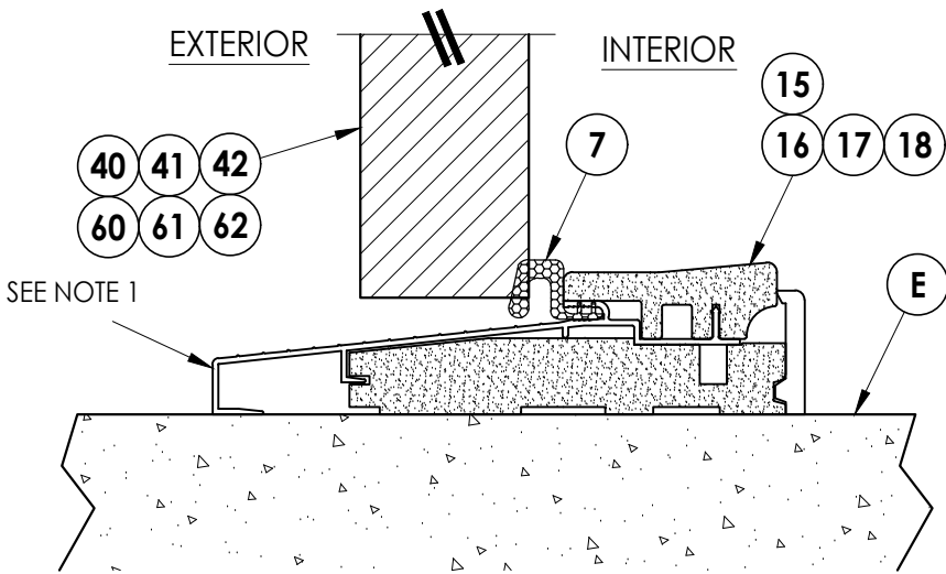
3 8 VERTICAL CROSS SECTION Outswing Sill
